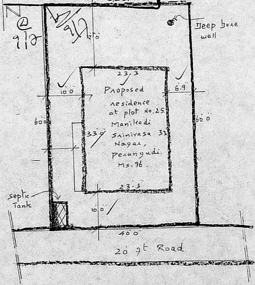
Site plan
